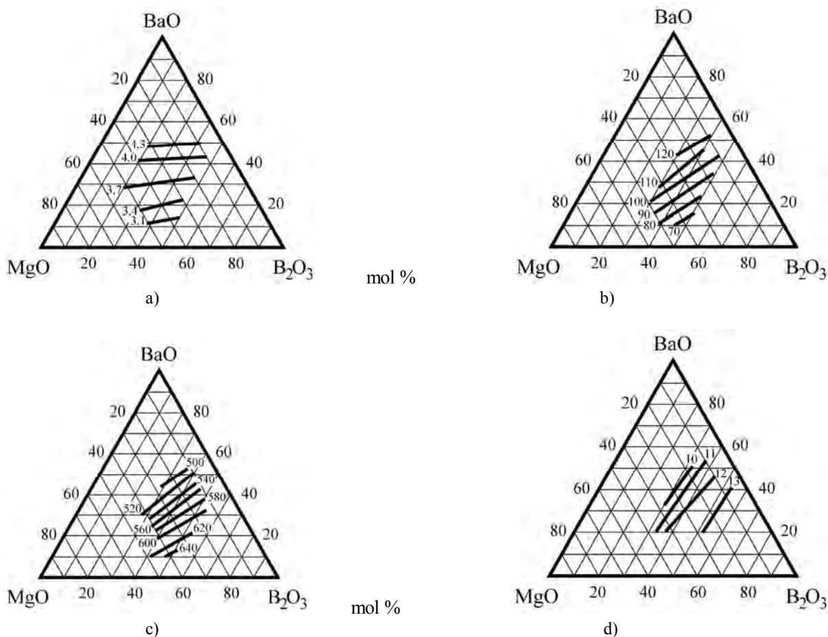
Fig. 2. Dependence of glasses properties in the researched field of MgO-BaO-B 2 O 3 system (contents of B 2 O 3 ≤ 50 mol %) of their chemical composition: density d , g/cm 3 (a); TCLE \alpha \cdot 10^7 , 1/grad (b); softening temperature T_s , °C (c) and logarithm of specific volume resistance at 573 K, Ohm·cm (d)
