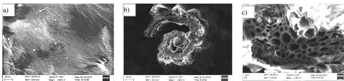
Fig. 5. SEM images of (a). Extracted chitosan – 1.00KX (b). AC derived from rice husks – 1.00 KX (c). AC derived from rice husks – 2.50 KX
