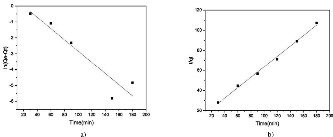
Fig. 10. (a) Pseudo-first-order (b) pseudo-second-order kinetic plots for the Pb(II) adsorption onto ACCHM (adsorbent dose = 0.05 g, pH = 5±0.2 initial concentration = 2 mg/L, agitation speed = 60 rpm, T=303±2 K)
