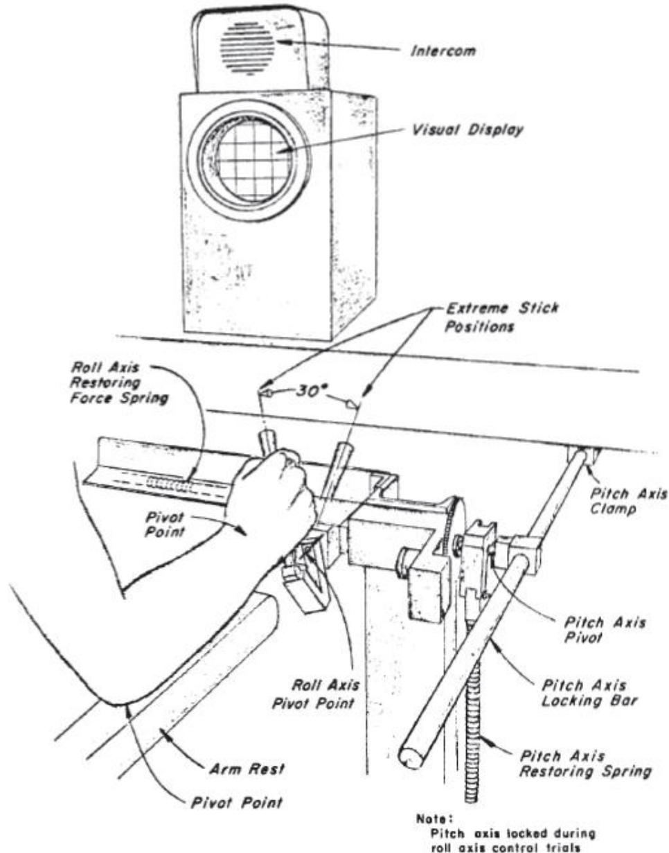
Fig. 1. Stick manipulator [7]
