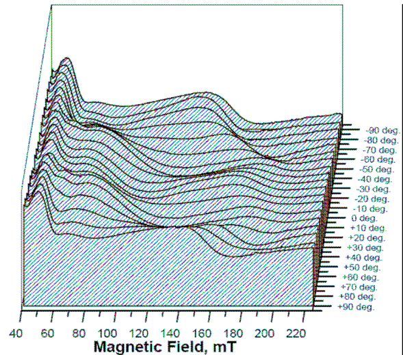
Fig. 3. The angular dependence of CR spectra for SQW p^+-n junction on \{100\} -Si. Rotation of the magnetic field \vec{H} in a \{100\} -plane perpendicular to a \{100\} -interface ( 0^\circ = \vec{H} \parallel \text{interface} , \pm 90^\circ = \vec{H} \perp \text{interface} ). T = 4 K, \omega = 9.45 GHz, \lambda = 577 nm.
