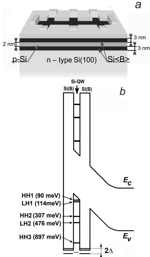
Fig. 1. Experimental structure of the Si nanosandwich prepared within the Hall geometry on the basis of an ultra-narrow p -type SQW confined by \delta -shaped barriers heavily doped with boron on an n -type Si (100) surface (Reproduced from [3]). The vertical gate is intended for controlling the 2D hole density and the intensity of spin-orbit interaction in QW.
