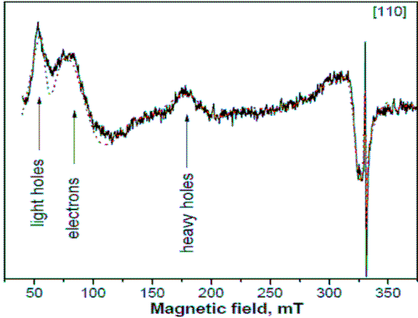
Fig. 4. The CR spectrum recorded at \vec{H} \parallel [110] . The dashed line is a fit with Eq. (1). Arrows stand for the peaks due to the light and heavy holes as well as electrons from the energy valleys with the long axis parallel and perpendicular to the magnetic field \vec{H} direction, respectively.
