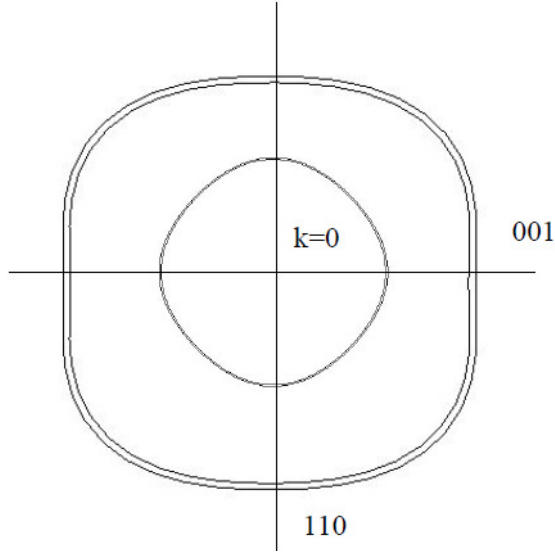
Fig. 6. The contours of the valence band constant energy surface in the (110) plane plotted for A, B, C parameters found in this work and taken from [12]. Outer contour for heavy hole corresponds to A = -4.002, B = 1.0, C = 4.025 , the inner contour is plotted for A = -4.0, B = 1.1, C = 4.1 . The contours for light holes for Si and SQW coincide.
