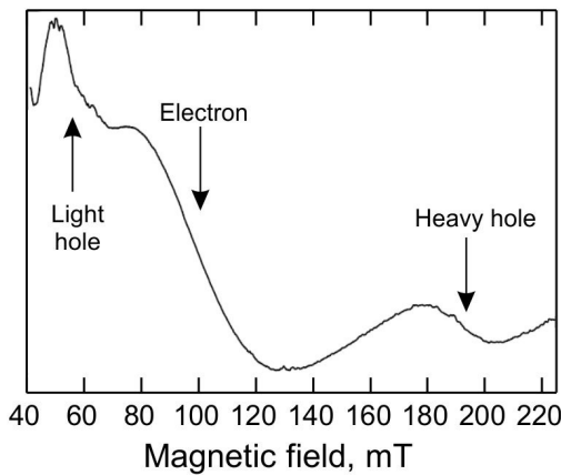
Fig. 2. Typical X-band CR spectrum for SQW p^+-n junction on \{100\} -Si, magnetic field \vec{H} within the \{110\} plane perpendicular to the \{100\} -interface ( \vec{H} \parallel \langle 100 \rangle - 20^\circ ) under illumination with light of the wavelength 577 nm. T = 4 K.
