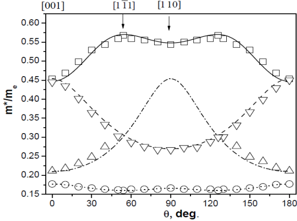
Fig. 5. The angular dependence of the effective masses for electrons m_{e1}^* ( \triangle ), m_{e2}^* ( \nabla ), light holes m_{lh}^* ( \circ ), and heavy holes m_{hh}^* ( \square ). Solid, dashed, dotted and dot-dashed curves are fits with Eq. (2) and Eq. (4) for electrons and holes, respectively.
