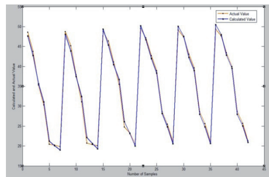
Fig. 6. Calculated values and the actual calibrated values of the test sample
