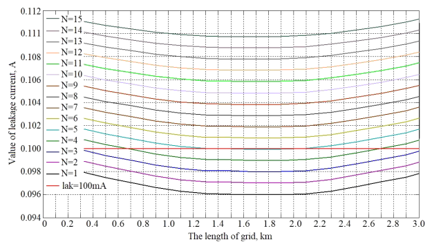
Fig. 13. The relation of I_r = f(L) corresponding to different connected apparatus ( N ) when there is 18 mH inductance compensation on earthing relay (the 3 rd tap change)
