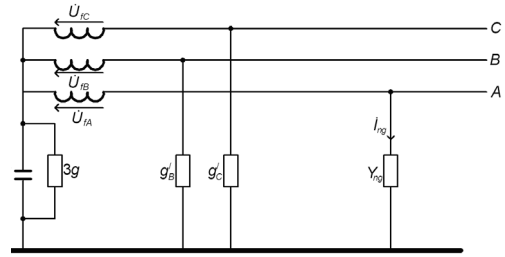
Fig. 6. Single line diagram of replaced circuit to compute earth current running through the human body
