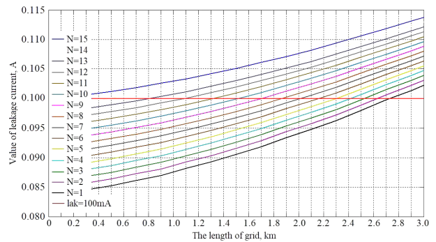
Fig. 12. The relation of I_r = f(L) corresponding to different connected apparatus ( N ) when there is 10 mH inductance compensation on earthing relay (the 2 nd tap change)
