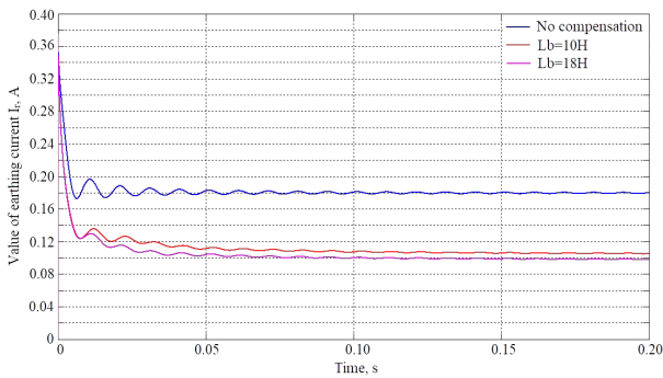
Fig. 10. Curves presented I_r = f(t) correspond to three compensation levels: red line I_r = f(t) corresponds to L = 10 H ; blue line I_r = f(t) corresponds to no compensation; bubble line I_r = f(t) corresponds to L = 18 H
