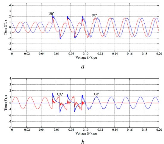
Fig. 17. Voltage waveform: a – on healthy phases with R_H connection; b – voltage waveform and U_0 wave-form on phase A (faulted phase)
