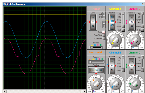
Fig. 11. AC voltage 3U_0 = 1 \text{ kV} (Cyan color) and output voltage across switching resistor
