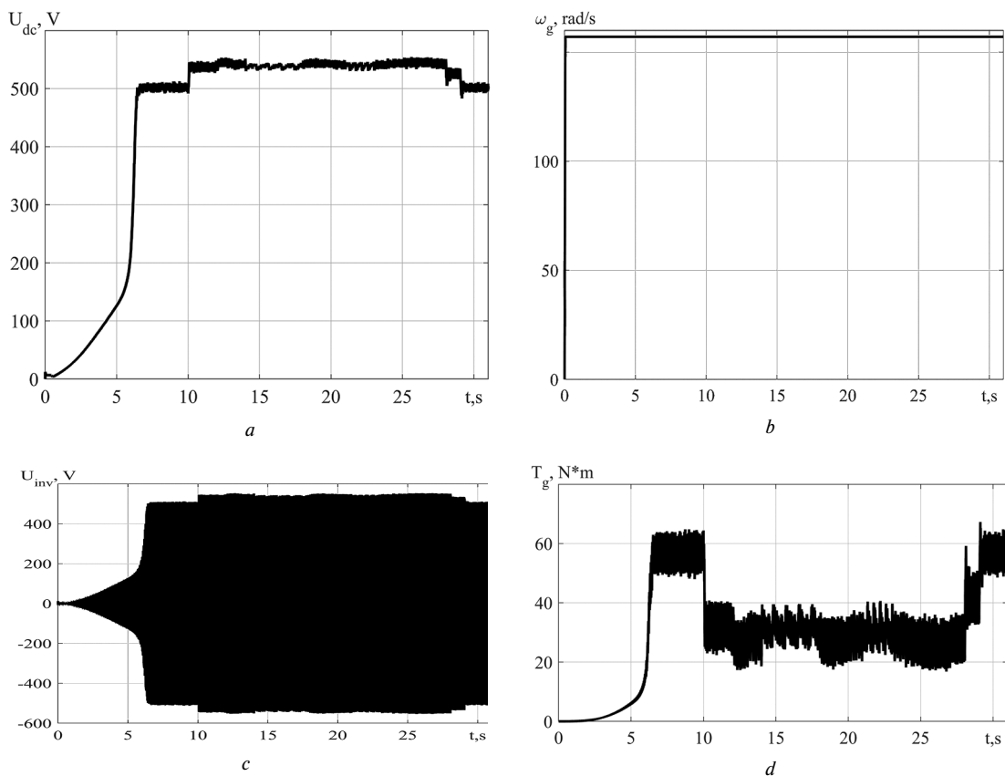
Fig. 8. Transients in the IG: a – DC-link voltage, U_{dc} ; b – rotor speed, \omega_g ; c – line-to-line inverter voltage, U_{inv} ; d – torque, T_g
