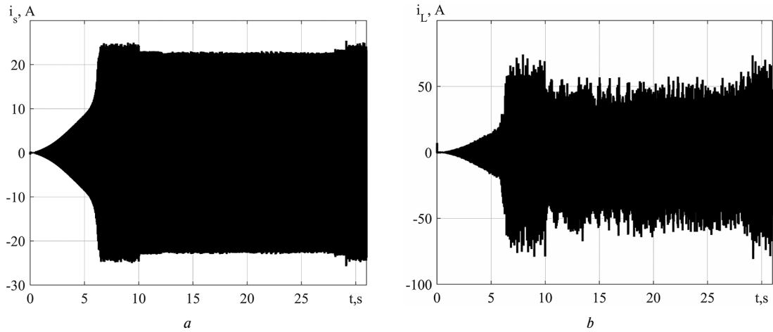
Fig. 7. Transients in the IG: a – stator line current, i_s ; b – line current, i_L
