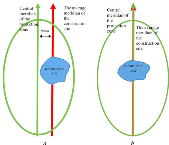
Fig. 2. The principle of central meridian selection: a – rules for choosing the central meridian of the UTM projection with the 30 zone; b – the central meridian of the UTM projection with the 30 zone in the average meridian coordinate system
