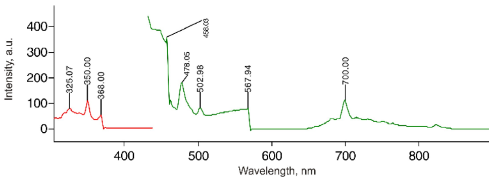
Fig. 3. Luminescence spectra of polycrystalline CVD ZnSe excited with a xenon lamp (polished surface; \lambda_{ex} = 325 \text{ nm} and \lambda_{ex} = 350 \text{ nm} ).
