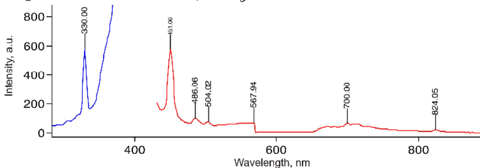
Fig. 2. Luminescence spectra of polycrystalline CVD ZnSe excited with a xenon lamp (polished surface; \lambda_{ex} = 330 \text{ nm} ).
