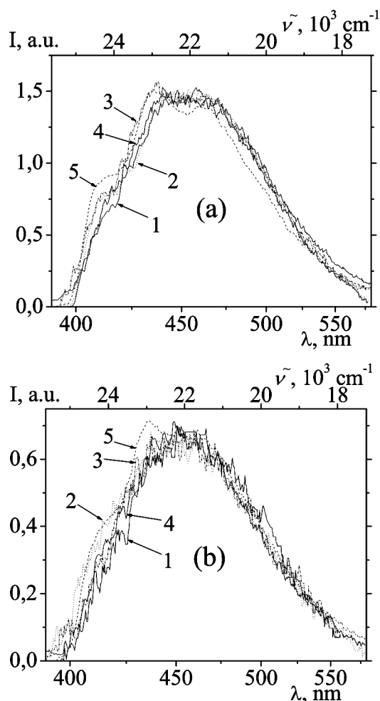
Fig. 4. Phosphorescence spectra at T = 4.2 \text{ K} (a) and T = 77 \text{ K} (b): DNA (1), d(CCCGGGTTTAAA) (2), poly(dAdT) 2 (3), d(ATC) (4), and d(AT) (5). Excitation at 300 nm. Water solutions, C = 10^{-4} \text{ M}
