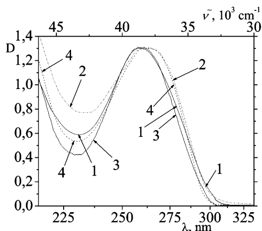
Fig. 2. Optical absorption spectra of DNA (1), d(CCCGGGTTTAAA) (2), RNA (3), and the sum (equimolar concentration) of the absorption spectra of nucleotides dAMP, dTMP, dGMP, and dCMP (4)
