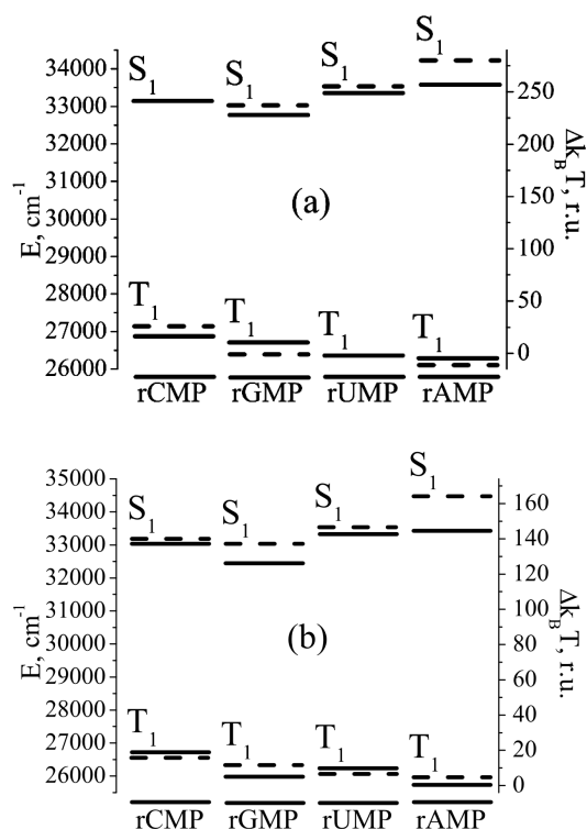
Fig. 3. Schemes of positions of the first singlet and triplet energy levels of the ribonucleotides (straight) and the deoxyribonucleotides (dash) at T = 4.2 K (a) and T = 77 K (b) (as an analog for rUMP, dTMP was given)
