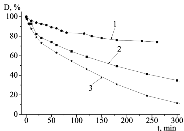
Fig. 7. Dependences of the optical density of the long-wave absorption spectrum maximum on the duration of UV-irradiation: 1 DNA, 2 tRNA, 3 oligo-RNA
