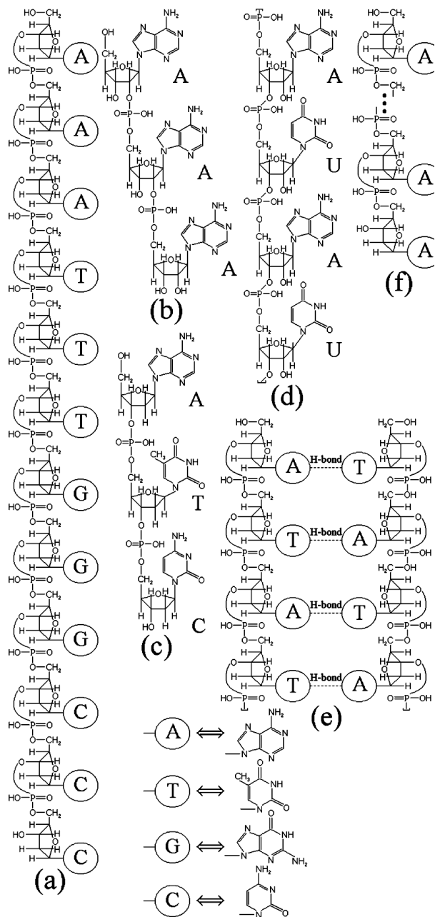
Fig. 1. Chemical formula of d(CCCGGGTTTAAA) (a), 2'5'A 3 (b), d(ATC) (c), single-stranded copolymer poly(rArU) (d), double-stranded copolymer poly(dAdT) 2 (e), d(AAAAAAAAAA) (f)
