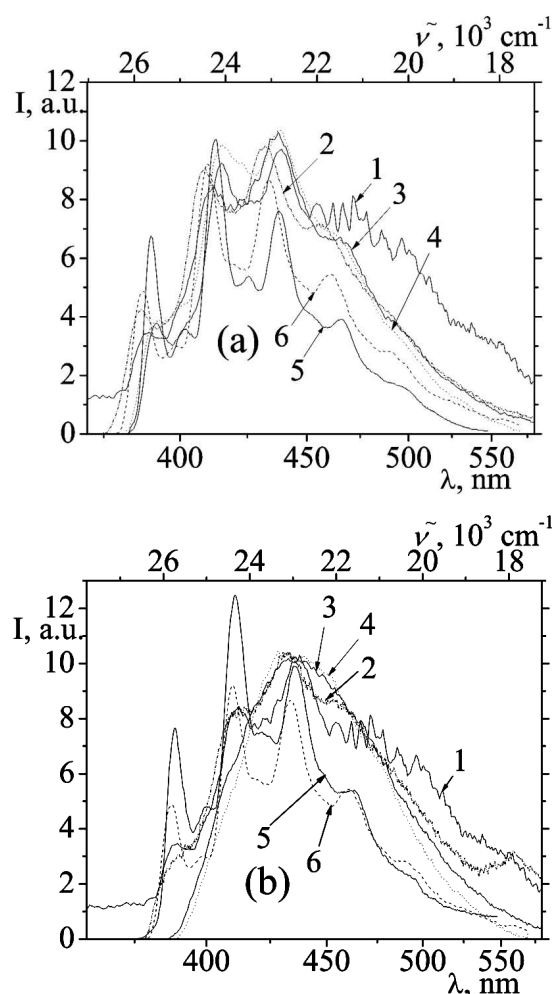
Fig. 5. Phosphorescence spectra at T = 4.2 \text{ K} (a) and T = 77 \text{ K} (b): tRNA (1), oligo-RNA (2), 2'5'A_3 (3), rAMP (4), d(AAAAAAAAAA) (5), and poly(rArU) (6). Excitation at 260 nm. Water solutions, C = 10^{-4} \text{ M}
