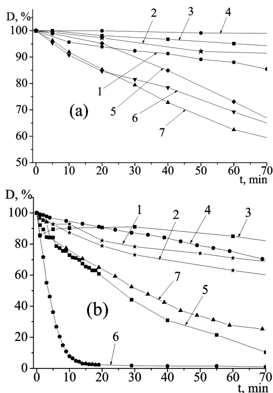
Fig. 6. Dependences of the optical density of the long-wave absorption spectrum maximum (a): 1 DNA, 2 d(CCCGGGTTTAAA), 3 poly(dAdT) 2 , 4 dAMP, 5 dCMP, 6 dTMP and 7 dGMP, (b): 1 tRNA, 2 oligoRNA, 3 2'5'A 3 , 4 rAMP, 5 rCMP, 6 rUMP, and 7 rGMP on the duration of UV-irradiation (the value of optical density is in from an intact value of the non-damaged sample)
