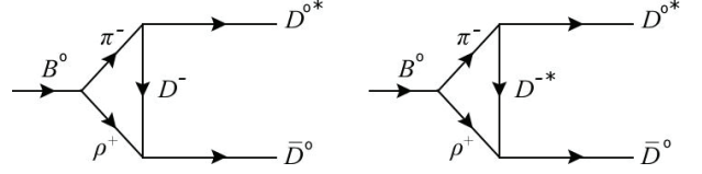
Fig. 7. HLL diagrams for the long-distance t -channel contribution to B^0 \rightarrow D^{0*} \bar{D}^0
