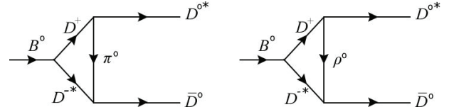
Fig. 3. HLL diagrams for the long-distance t -channel contribution to B^0 \rightarrow D^{0*} \bar{D}^0
