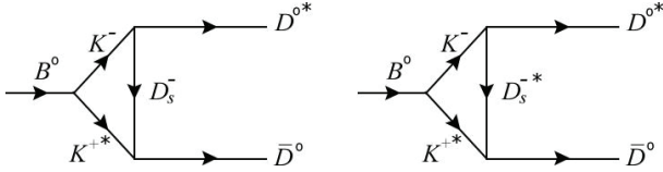
Fig. 5. HLL diagrams for the long-distance t -channel contribution to B^0 \rightarrow D^{0*} \bar{D}^0
