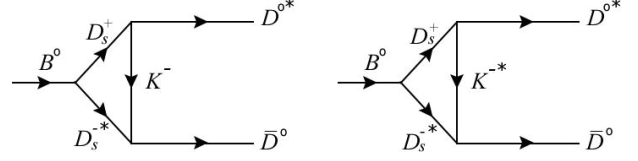
Fig. 11. HLL diagrams for the long-distance t -channel contribution to B^0 \rightarrow D^{0*} \bar{D}^0
