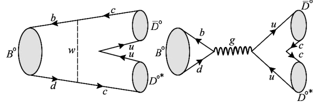
Fig. 1. Some quark diagrams illustrating the process B^0 \rightarrow D^{0*} \bar{D}^0
