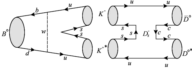
Fig. 4. Quark level diagram for B^0 \rightarrow K^{+*} K^-
