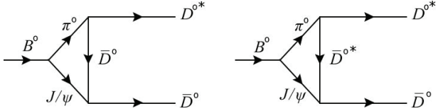
Fig. 13. HLL diagrams for the long-distance t -channel contribution to B^0 \rightarrow D^{0*}\bar{D}^0
