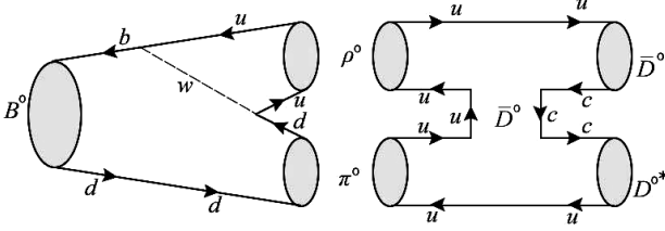
Fig. 8. Quark level diagram for B^0 \rightarrow \rho^0 \pi^0
