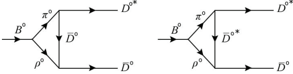
Fig. 9. HLL diagrams for the long-distance t -channel contribution to B^0 \rightarrow D^{0*} \bar{D}^0
