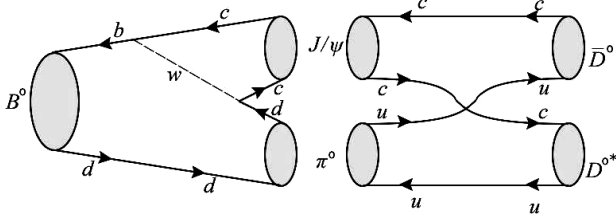
Fig. 12. Quark level diagram for B^0 \rightarrow J/\psi\pi^0
