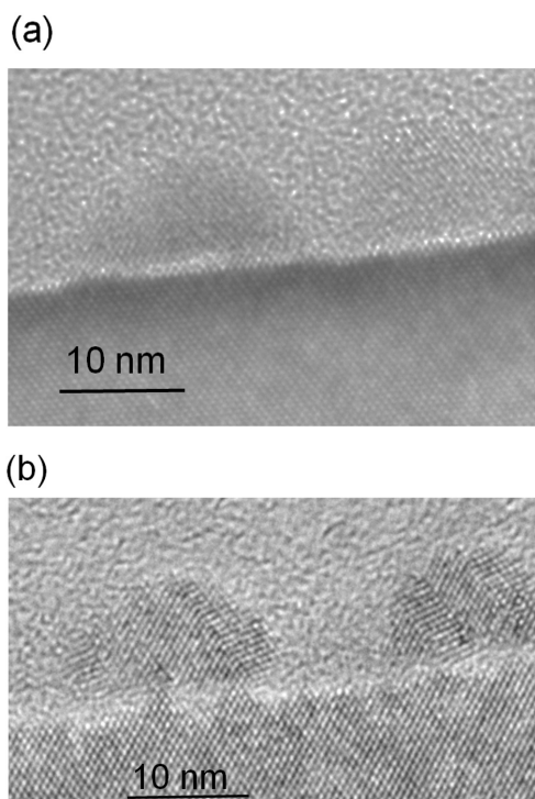
Fig. 2. HRTEM images of Ge nanoclusters grown on silicon oxide
