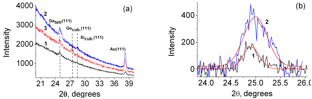
Fig. 3. a ) X-ray diffraction spectra for samples recorded at the incident angle \omega = 0.5^\circ . 1 – as-grown sample with Ge nanoclusters grown on chemically oxidized Si(100); 2 – with 8 MLs of Si; 3 – structure with Ge nanoclusters covered by a 25-nm-thick Si layer. b ) Peaks subtracted from spectra for the as-grown sample with Ge nanoclusters and the sample with 8 MLs of Si
