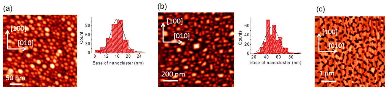
Fig. 1. a ) AFM image of the surface with Ge nanoislands, grown on the surface of a \text{SiO}_2 film and distributions of nanoclusters over base diameters (structure A); b ) the same for the surface modified by the deposition of Si on the structure with Ge nanoislands (structure B); c ) AFM image of the surface of structure C with Ge nanoclusters covered by a 25-nm-thick Si layer
