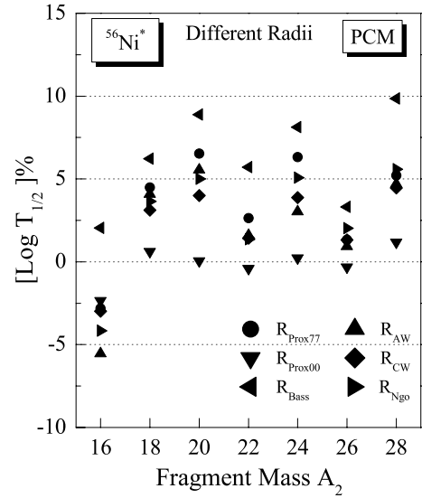
Fig. 9. Percentage variation of \log T_{1/2} for different forms of radii with PCM only
