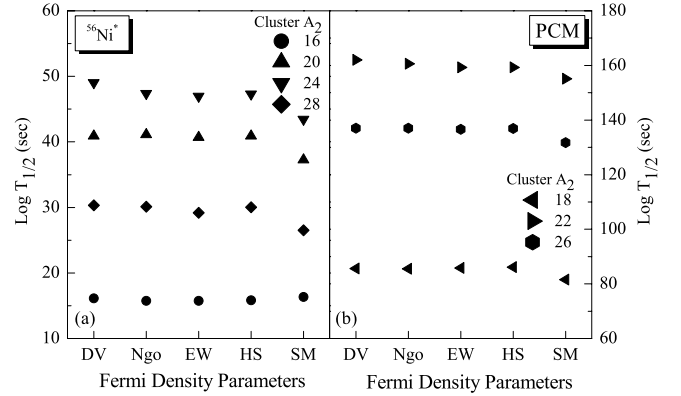
Fig. 4. Variation of \log T_{1/2} (s) using different density parameters for PCM
