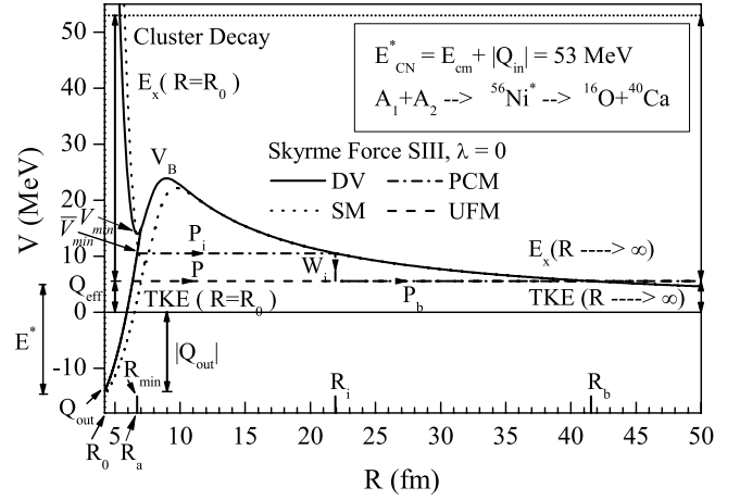
Fig. 2. Scattering potential V(R) (MeV) for the cluster decay of ^{56}\text{Ni}^* into ^{16}\text{O} + ^{40}\text{Ca} channel for different Fermi density parameters. The distribution of compound nucleus excitation energy E_{\text{CN}}^* at both the initial ( R = R_0 ) and asymptotic ( R \rightarrow \infty ) stages and Q -values are shown. The decay path for both PCM and UFM models is also displayed
