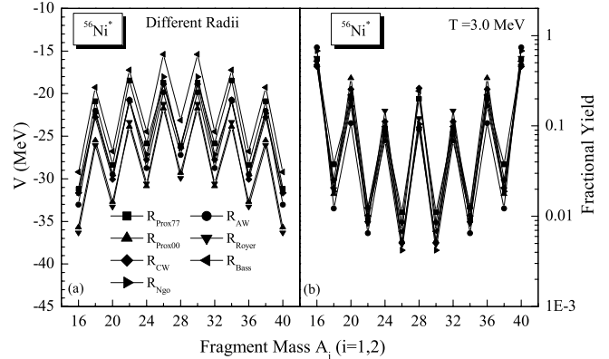
Fig. 7. Same as in Fig. 3, but for different radii
