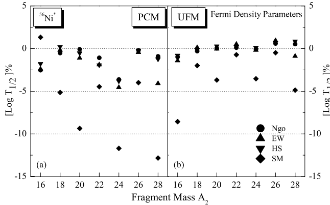
Fig. 5. Percentage variation of \log T_{1/2} for different Fermi density parameters w.r.t. DV parameters
