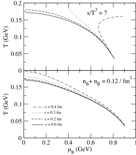
Fig. 2. The effect of excluded volume corrections on the constant n_B + n_{\bar{B}} (bottom) and constant s/T^3 (top) freeze-out criterion. This figure is taken from the preprint J. Cleymans, H. Oeschler, K. Redlich, and S. Wheaton, arXiv:hep-ph/0511094v2 of Ref. [8] in order to demonstrate the unrealistic behavior of the chemical freeze-out criterion s/T^3 = 7 , if the hard core repulsion is taken into account. For the hard core radius R = 0.3 fm, which was used in [2–4] to fit the data, the chemical freeze-out criterion s/T^3 = 7 does not work
