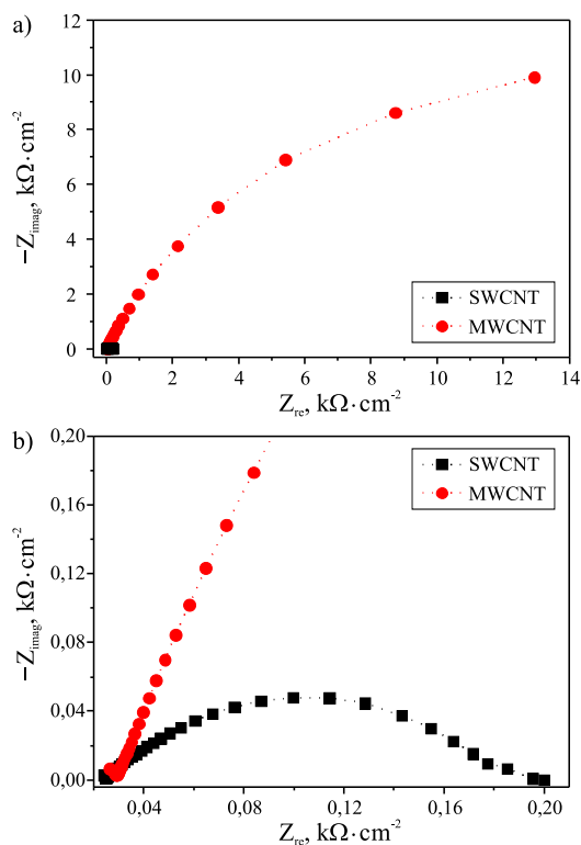
Fig. 4. EIS spectra recorded for aqueous SWCNT and MWCNT suspensions (1.0 KCl) on a GC electrode ( 0.24 \text{ cm}^2 ) in the frequency range 0.1 Hz–100 kHz (a); zoom of EIS spectra in the high frequency region (b)
