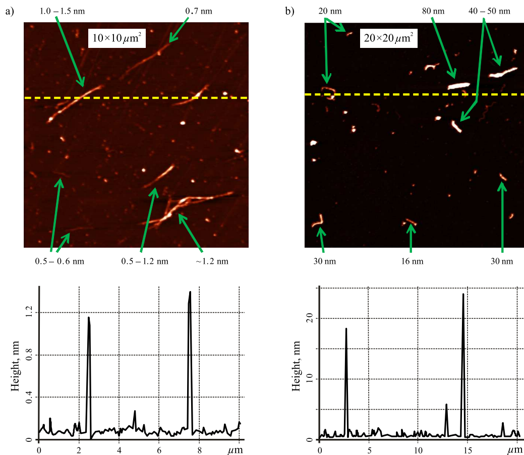
Fig. 2. AFM images of SWCNTs (a) and MWCNTs (b) deposited from an aqueous suspension (concentration: 5 \mu\text{g}/\text{ml} ) on the mica substrate (tapping mode). Topographic images for a given profile (dashed line) are shown on the top. The diameters of some CNTs are indicated by arrows
