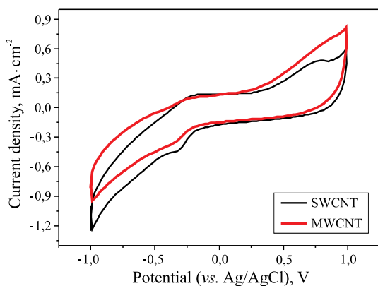
Fig. 3. CVs recorded for aqueous SWCNT and MWCNT suspensions (1.0 KCl) on a GC electrode ( 0.24 \text{ cm}^2 ) at v = 0.10 \text{ V} \cdot \text{s}^{-1}
