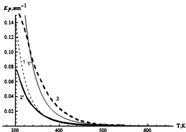
Fig. 2. Temperature dependences of the dimerization constant for the saturated vapors of heavy (1) and light (1') waters according to the results of work [19] and for heavy (2) and light (2') waters according to the calculations by formula (10)
