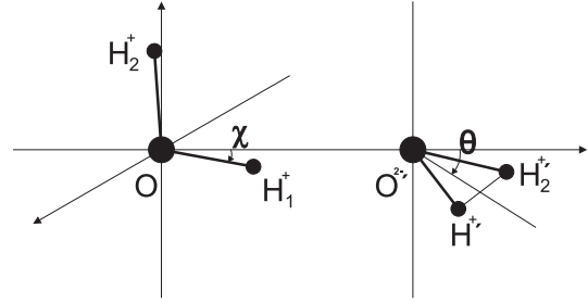
Fig. 1. Equilibrium configuration of a water dimer
