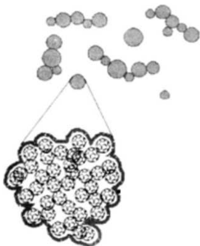
Fig. 6. Structure model for the fluid mixture “water–fullerene C 60 ” proposed on the basis of neutron experiment results [62]
