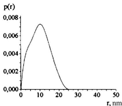
Fig. 7. Size distribution function as a result of the simulation of neutron scattering in the system C 60 –NMP–H 2 O, by using the method of indirect Fourier transformation [62]
