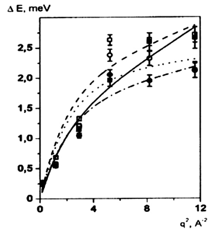
Fig. 1. Dependence of the quasielastic peak broadening \Delta E on the squared scattering vector q^2 for an aqueous suspension of membranes
