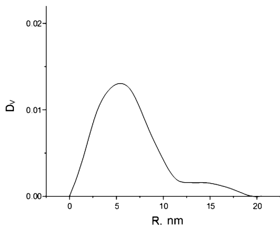
Fig. 5. Size distribution function of particles in a ferrofluid [44]
