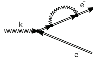
Fig. 3. Feynman diagram for the process of e^-e^+ pair photoproduction through the mass operator
