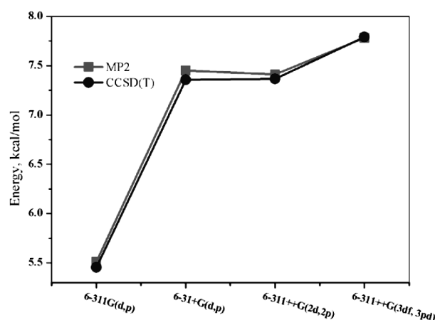
Fig. 2. Graphical presentation of the stabilization energies of the \text{H}_2\text{CO}\cdots\text{HF} complex calculated in the CCSD(T) and MP2 methods as a function of the various basis sets
