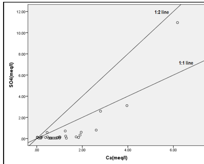
Fig. 8. Ca 2+ vs. SO 4 2- scatter diagram
