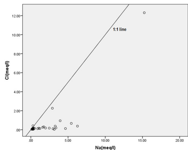
Fig. 10. Relationships between Na + and Cl -
