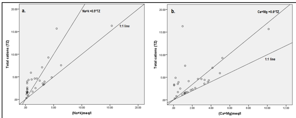
Fig. 9. a: Na + +K + vs Total cations (TZ); b: Ca 2+ +Mg 2+ vs Total cations (TZ)
