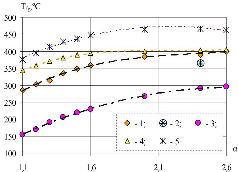
Fig. 3. Comparison of experimental and calculated values of flue gases temperature: 1 – by the formula (1) with the coefficients in the correction (2) c = 2,4 , m = 0,68 ; 2 – experimental data; 3 – by (1) with c = 5,7 , m = 0,6 ; 4 – by the formula, suggested by the authors on the basis of the experiment (3); 5 – by the formula (1) without taking into account the correction.
