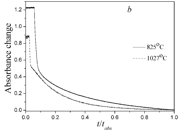
Fig. 7. The kinetics of the absorbance changes of G 1 film during reducing (a) and oxidizing (b) annealing at different temperatures. For a better visualization, the time is normalized for each curve to the full time of observation t_{obs} ; figure a: t_{obs} = 146.4 min. at 825 °C, 46.9 min. at 1027 °C; figure b: t_{obs} = 46.9 min. at 825 °C, 36 min. at 1027 °C
