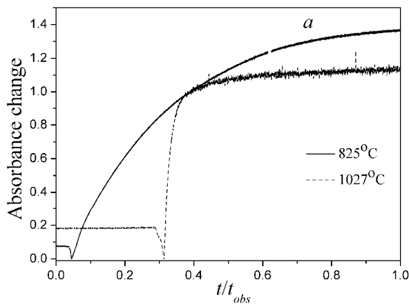
Fig. 7. The kinetics of the absorbance changes of G 1 film during reducing (a) and oxidizing (b) annealing at different temperatures. For a better visualization, the time is normalized for each curve to the full time of observation t_{obs} ; figure a: t_{obs} = 146.4 min. at 825 °C, 46.9 min. at 1027 °C; figure b: t_{obs} = 46.9 min. at 825 °C, 36 min. at 1027 °C
