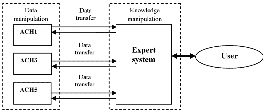
Figure 3 –Logical structure of five-tier ultra-wideband WDR filter KB CAD system
