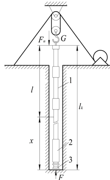
Fig. 1. Modeled scheme of drill string: 1 – drill string; 2 – immersed engine; 3 – bit
