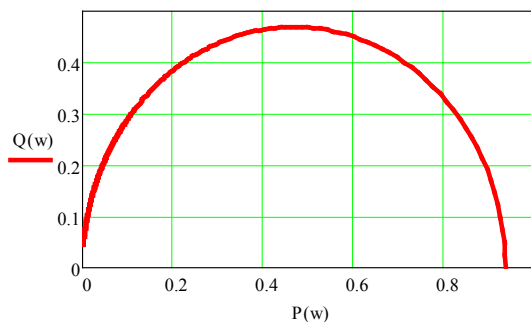
Fig. 6. APC chart of the forming filter for axial effort F at manual control
