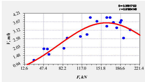
Fig. 2. Informational models for the relation between mechanical drilling speed with axial effort: a – quadratic; b – inversely-quadratic; c – Gaussian
