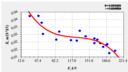
Fig. 3. Informational polynomial model of 3rd degree for coefficient k
