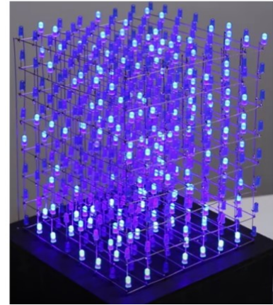
Fig. 4. Layout of devices for presenting volumetric stimuli – LED cube of 8x8x8 LEDs
