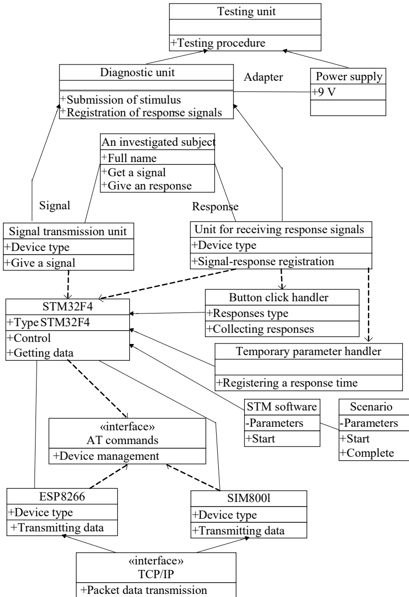
Fig. 3. Class diagram of the testing unit and the data processing and transmission unit
