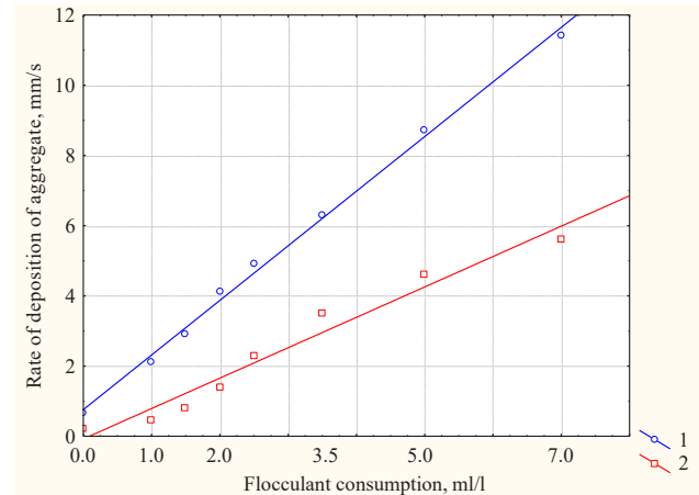
Fig. 10. Dependence of the rate of deposition of floccules after the introduction of coagulant (in the amount of 250 mg/l) and flocculant: 1 – after introduction of reagents; 2 – after mechanical influence by stirring for 40 s
