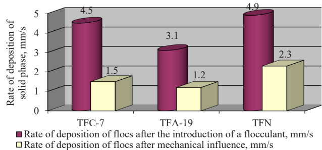
Fig. 7. Rate of deposition of solid phase after the introduction of coagulant (in the amount of 250 mg/l) and flocculants (in the amount of 250 ml/l) before and after mechanical influence by stirring for 40 s
