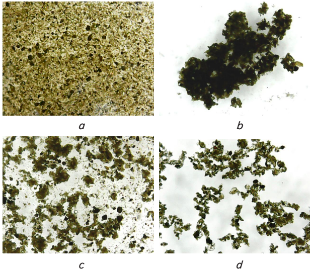
Fig. 8. Images after flocculation and destruction of flocs during mechanical influence: a – dispersed system in a drop of wastewater before the introduction of reagents; b – the view of flocs after aggregation; c – the view of flocs cells formed by TFN flocculant after mechanical influence; d – the view of flocs cells formed by TFC-7 flocculant after mechanical influence
