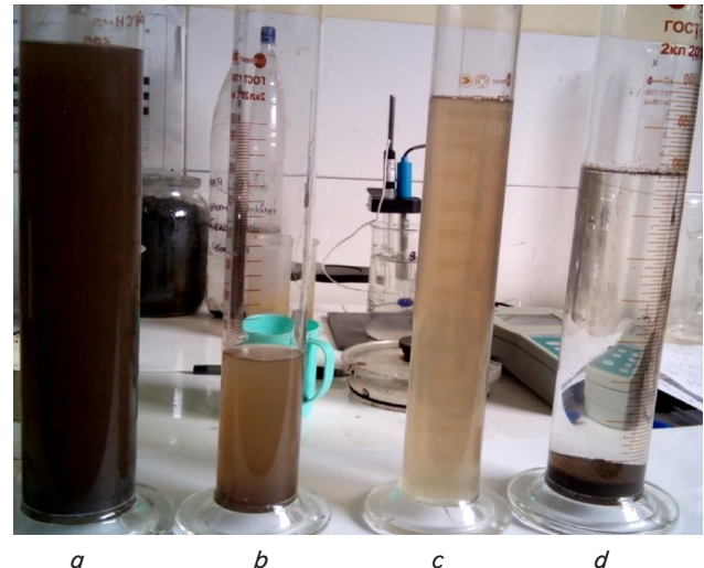
Fig. 6. Comparative analysis of the effectiveness of treatment of wastewater of chips production: a – settling, b – filtration; c – coagulation and flocculation with subsequent settling; d – centrifugation
