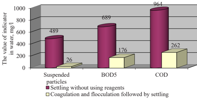
Fig. 9. Comparative analysis of the effectiveness of wastewater treatment by coagulation-flocculation method (coagulant consumption – 250 mg/l, consumption of flocculant solution – 2.5 ml/l)
