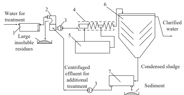
Fig. 11. Production circuit of treatment of wastewater after washing potatoes for making chips: 1 – tank-storage of wastewater; 2 – filter; 3 – pump; 4 – flocculator; 5 – station of preparation and dosage of reagents (coagulants and flocculant); 6 – thin-layer settling tank; 7 – centrifuge for dehydration of condensed sludge
