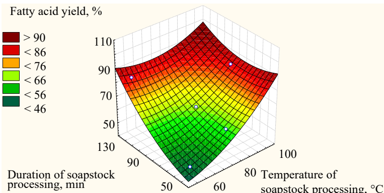
Fig. 2. Dependence of the fatty acid yield on the temperature and duration of soapstock processing with sulfuric acid (response surface)
