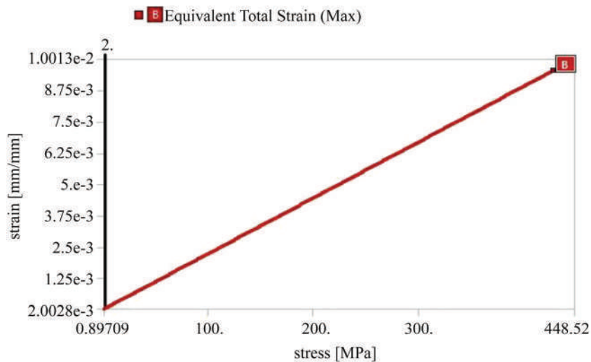
Fig. 9. Stress-strain relationship for magnesium alloy
