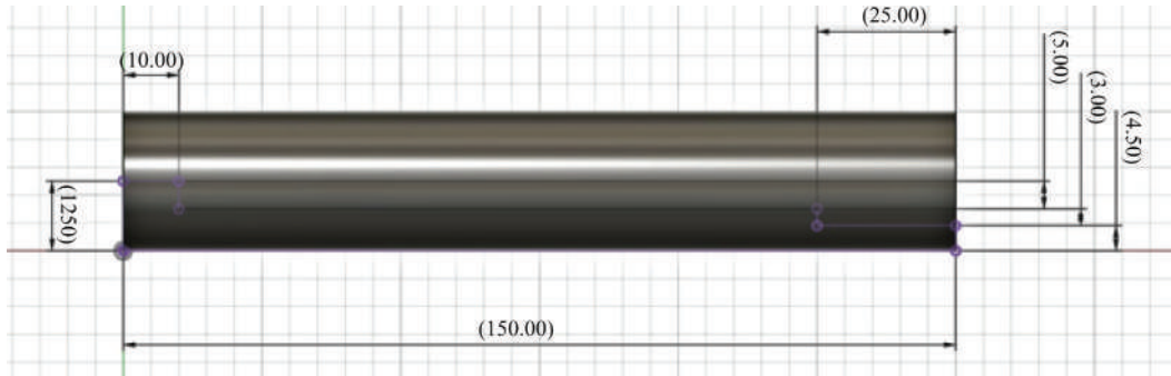
Fig. 1. 3D dimensional design of the fixed die
