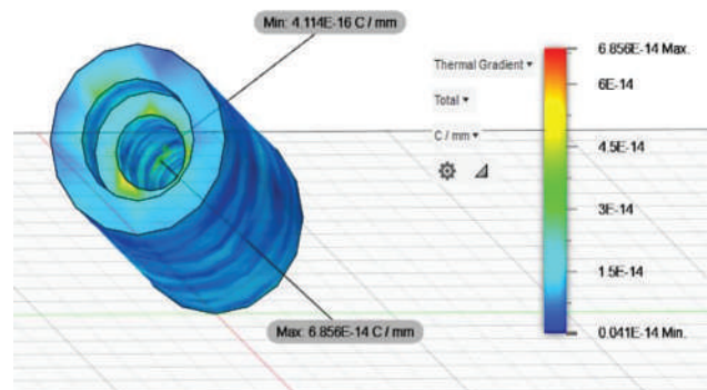
Fig. 5. Temperature distribution of magnesium alloy
