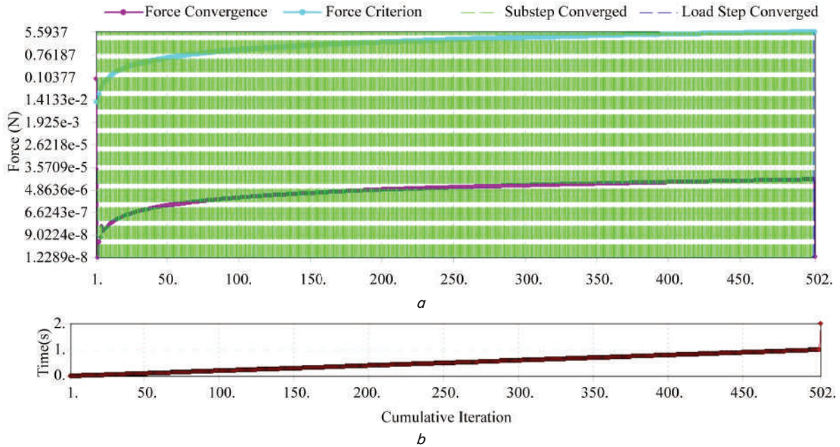
Fig. 8. Structural analysis of: a – convergence of force; b – iteration for magnesium alloy
