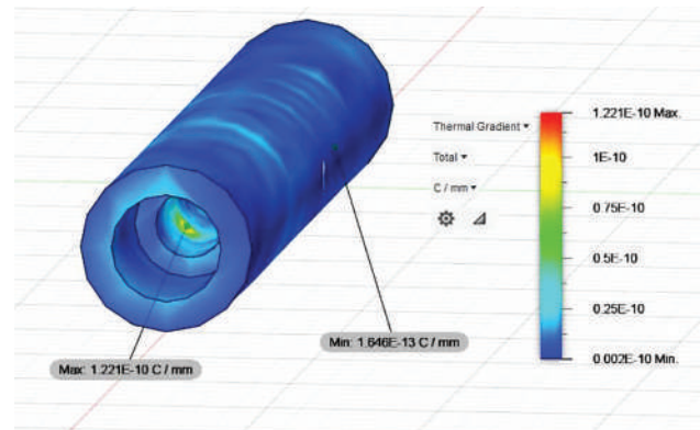
Fig. 4. Temperature distribution of aluminum alloy
