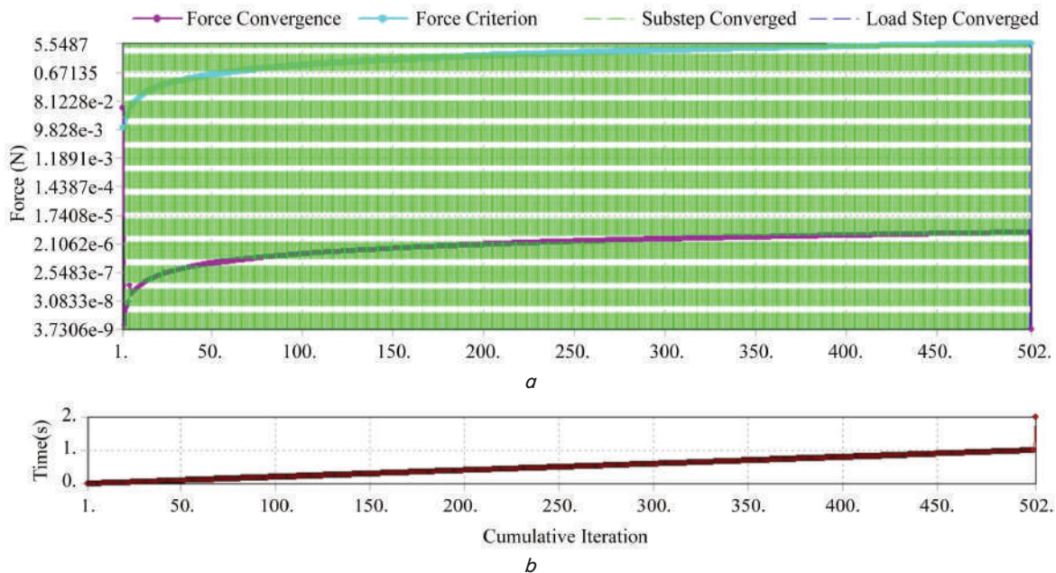
Fig. 6. Structural analysis of: a – convergence of force; b – iteration for aluminum alloy
