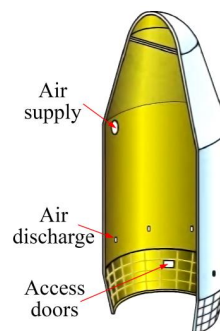
Fig. 2. Scheme of air supply to the main fairing during thermostating [2]
