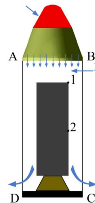
Fig. 4. Estimated «scheme No. 1»: 1–2 – surface of special «sensitivity»; 3 – additional air supply zone; ABCD – estimated region
