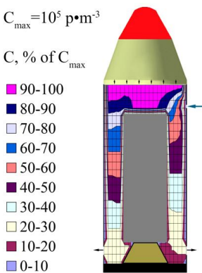
Fig. 6. Dust concentration field in the main fairing when the satellite is located according to the «scheme number 1», the second scenario (additional blowing)
