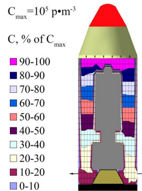
Fig. 9. The field of dust concentration in the main fairing when the satellite is located according to the «scheme number 2»
