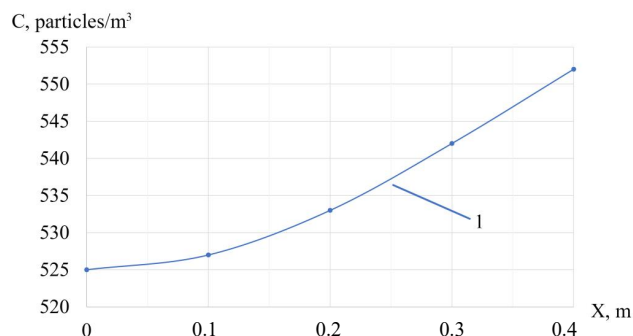
Fig. 11. The number of settled dust particles on the vertical «sensitive» surface 3–4 per day
