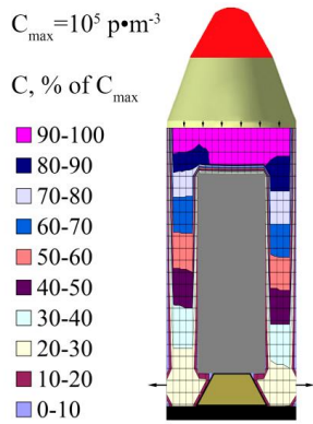
Fig. 5. The field of dust concentration in the main fairing when the satellite is located according to the «scheme number 1», the first scenario
