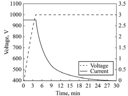
Fig. 11. Dynamics of current and voltage at electro-adhesive connection (own drawing)
