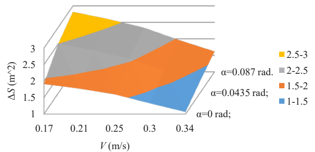
Fig. 10. Graph of dependence of the change in the useful area of leather on the rate of its feeding
