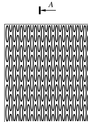
Fig. 5. Scheme of uniform arrangement of rollers of the guiding device (top view)
