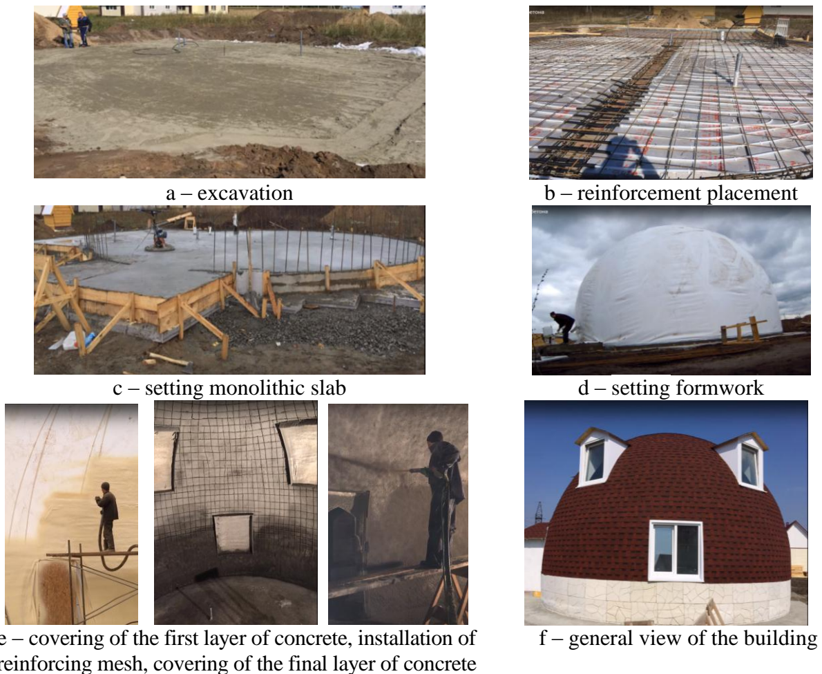
Fig. 3. Photo-fragments of the organizational and technological sequence of works
