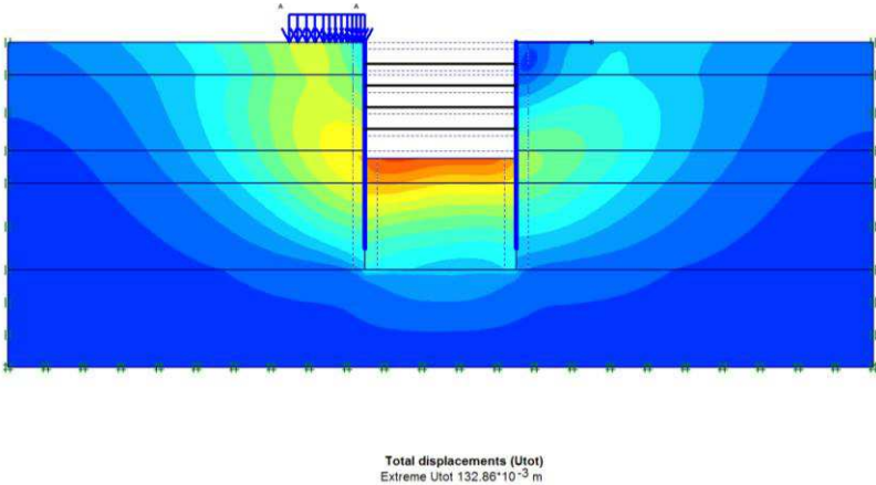
Fig. 11. Shaded displacement at 6 th excavation
