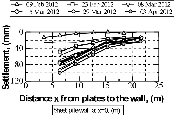
Fig. 10. Monitoring data of surface settlement at plates SP-01 to SP-07
