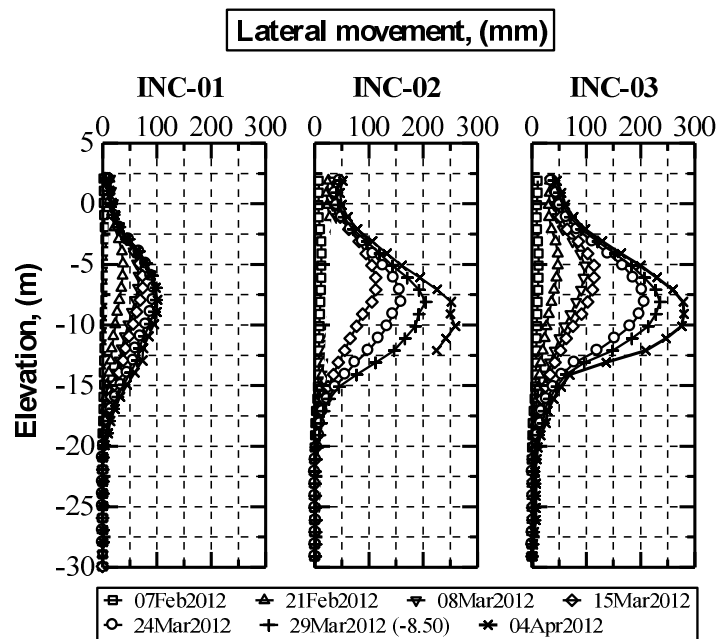
Fig. 9. Monitoring data of lateral movement at all three inclinometers
