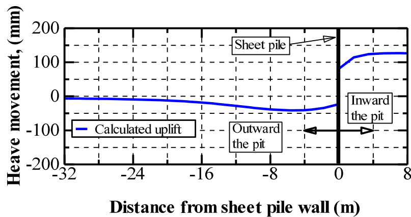
Fig. 13. Uplift at bottom of the excavation pit
