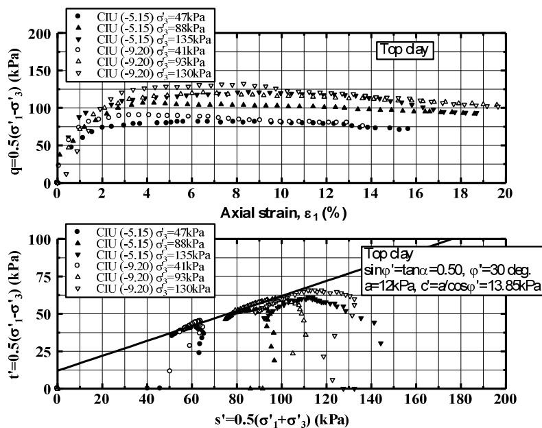
Fig. 6. Triaxial test results for top soft clay
