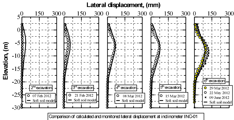
Fig. 14. Comparison of calculated and monitored lateral movement at inclinometer INC-01
