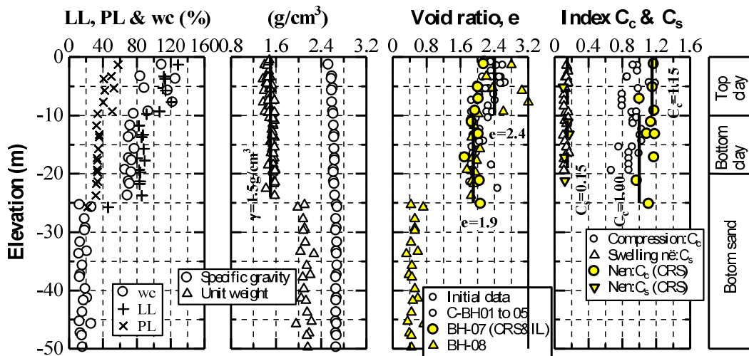
Fig. 3. Physical mechanical properties
