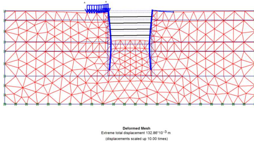
Fig. 12. Deformed mesh at 6 th excavation
