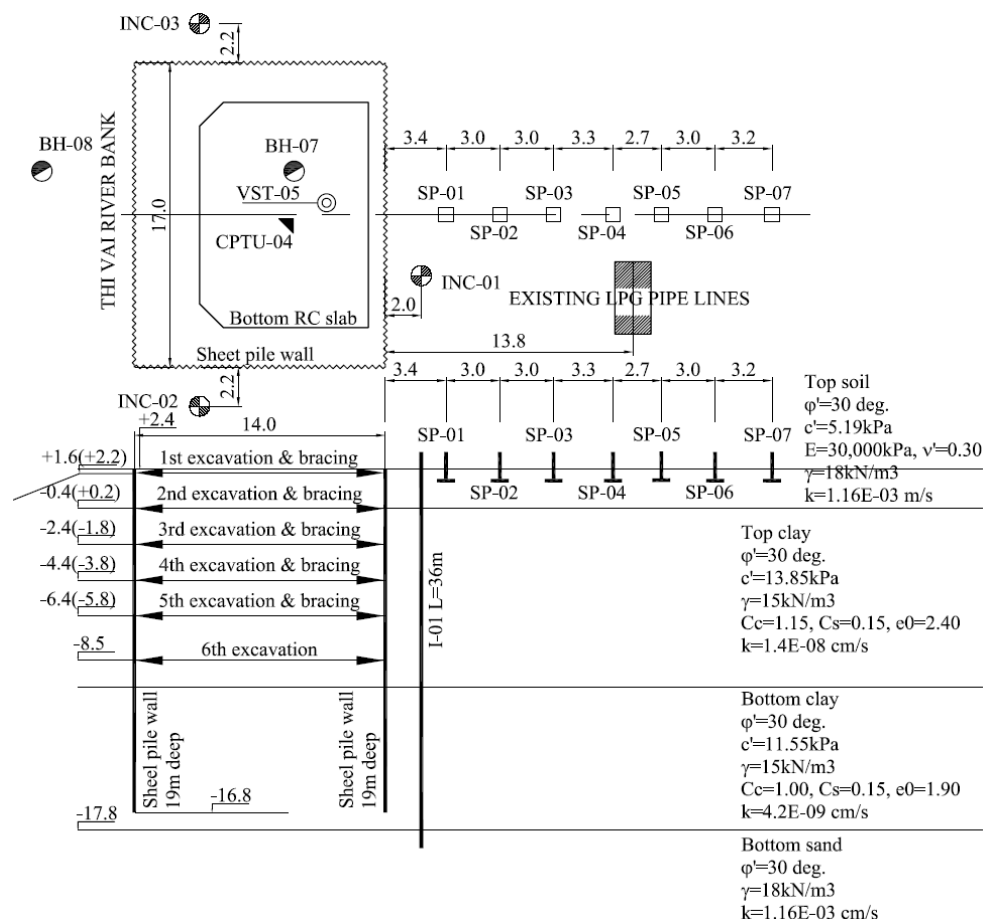
Fig. 8. Arrangement of monitoring instrumentations (Dimension in m)
