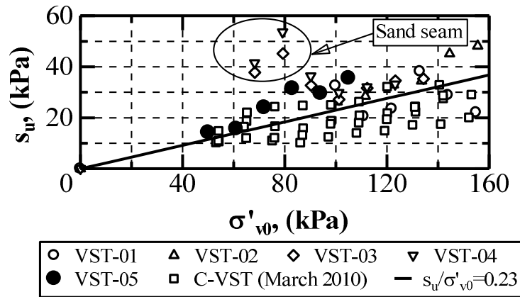
Fig. 5. s_u vs. over-burdened stress ratio
