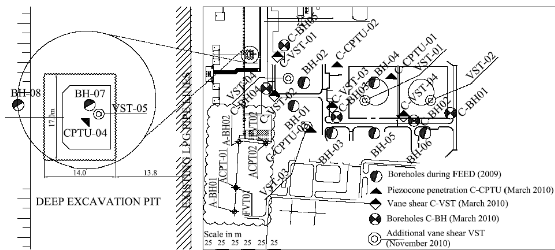
Fig. 2. Layout plan of soil investigation for the project site
