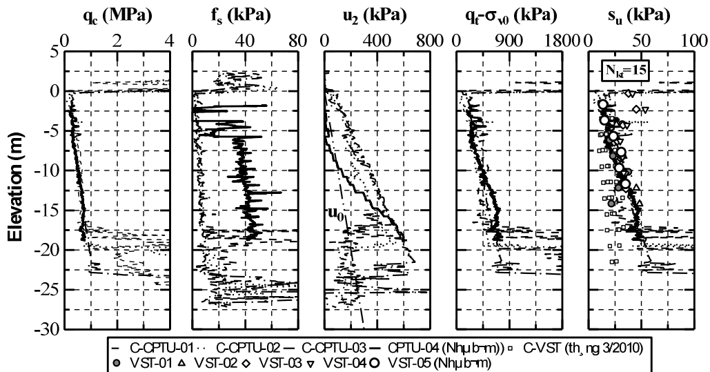
Fig. 4. Piezocone penetration and field vane shear test results
