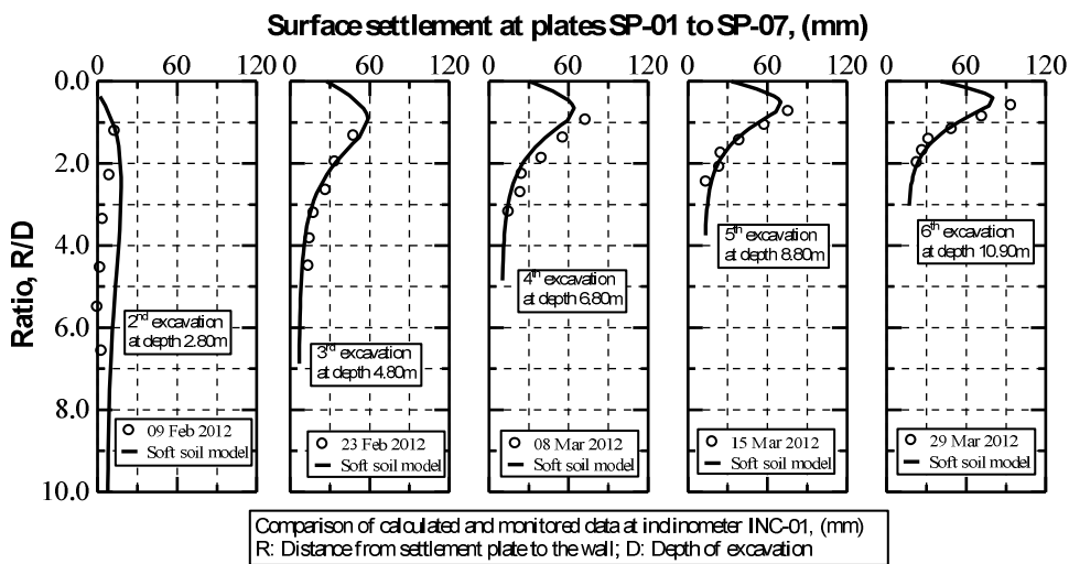
Fig. 15. Comparison of calculated and monitored ground loss from the face of sheet pile wall
