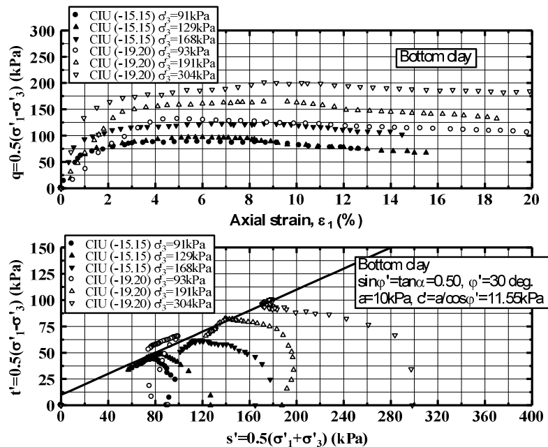
Fig. 7. Triaxial test result for bottom soft clay
