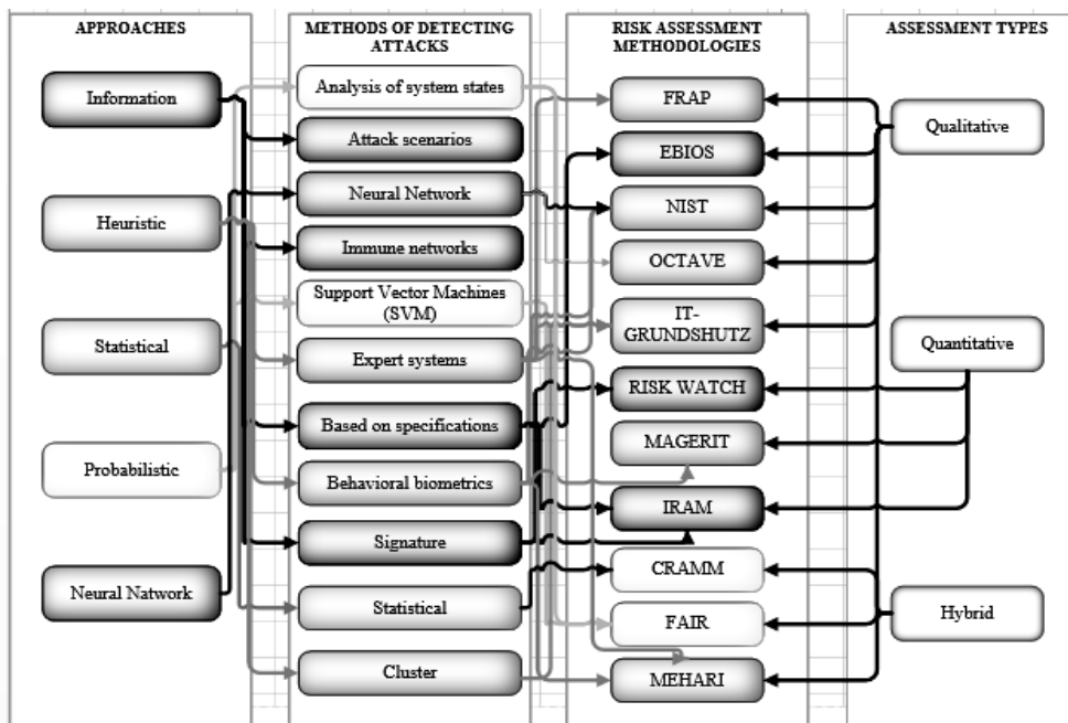
Fig. 1. The relation between methods of detecting attacks and risk assessment methods
