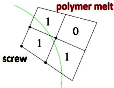
Fig. 2. Presentation of “Inside” Field for a 2D Finite Element
