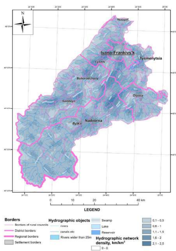
Fig. 4. Map model of hydrological network density in Bystrytsia river basin
