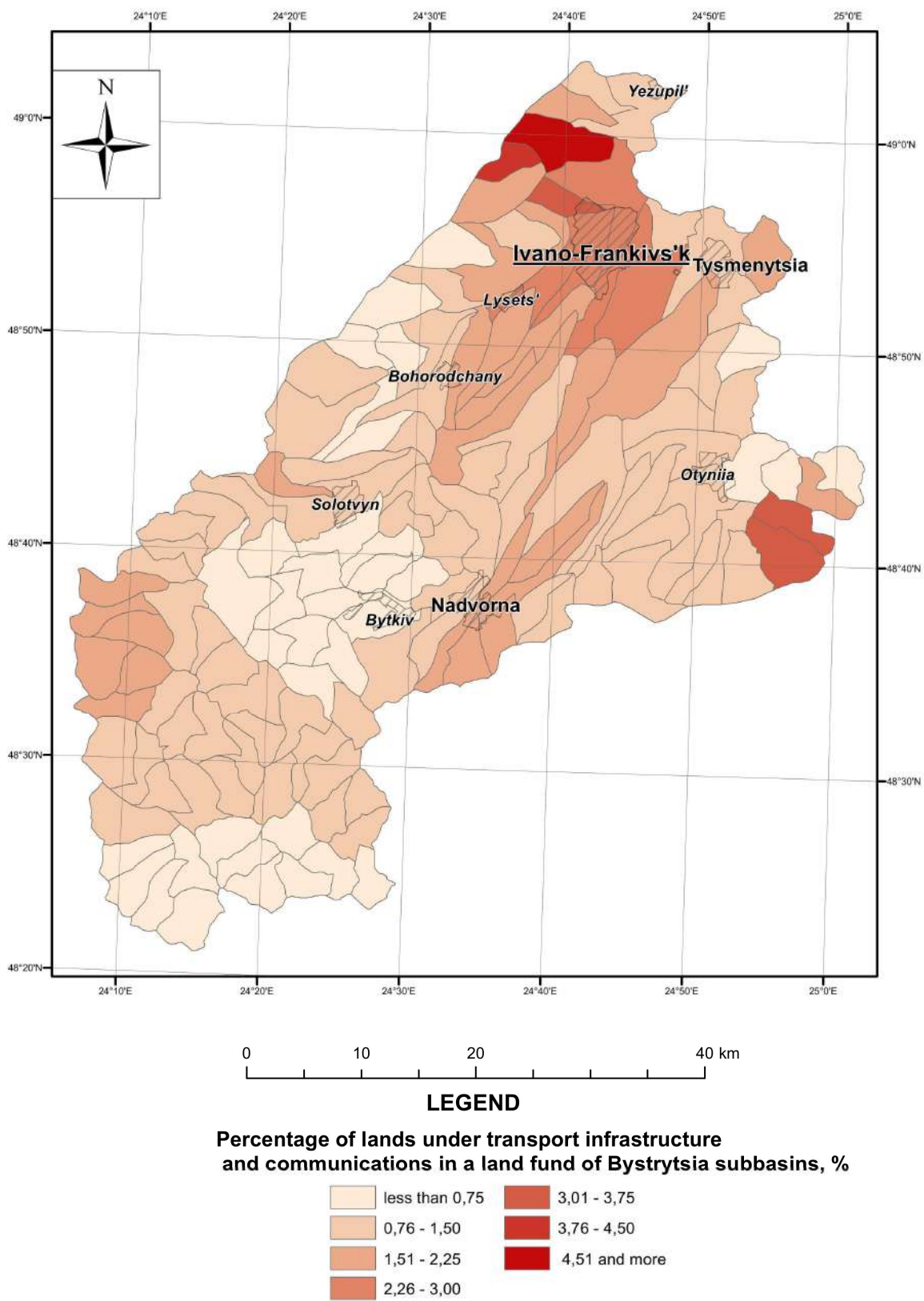
Fig. 8. Share of land of transportation and infrastructure land use in land use structure of Bystrytsia RBS sub-basins
