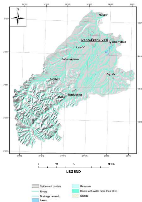
Fig. 3. Map model of hydrological network in Bystrytsia river basin
