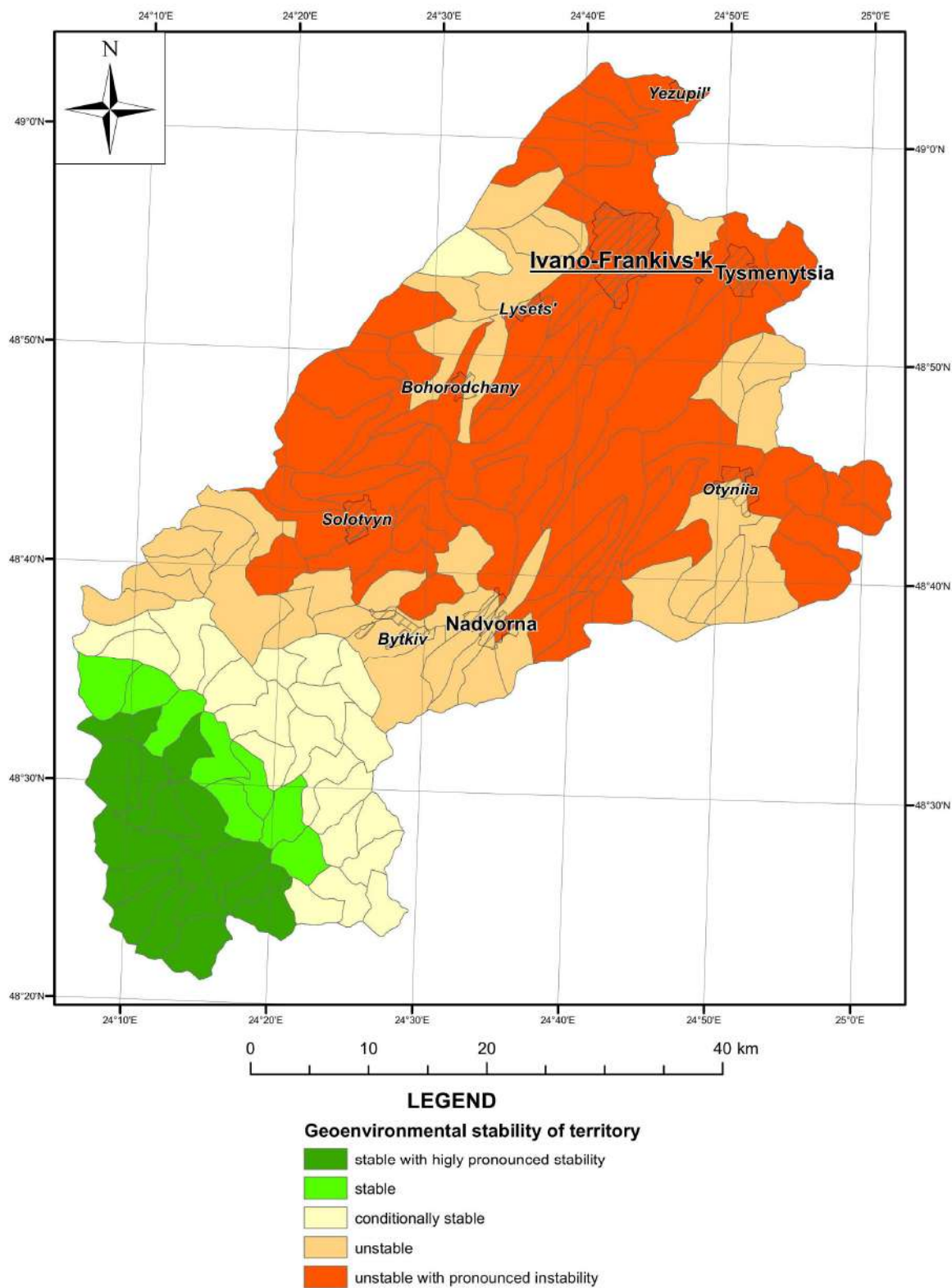
Fig. 9. Assessment of the level of geoenvironmental stability for Bystrytsia RBS sub-basins (calculated with method proposed by E. Klementova, V. Heinige, 1995)
