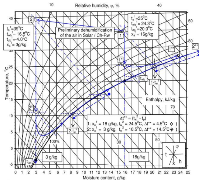
Figure 4 – Performance analysis of the Ch-Rw ( l = G_a/G_{w\Sigma} = 1.0 and l^* = G^1/G^2 = 1.0 )
