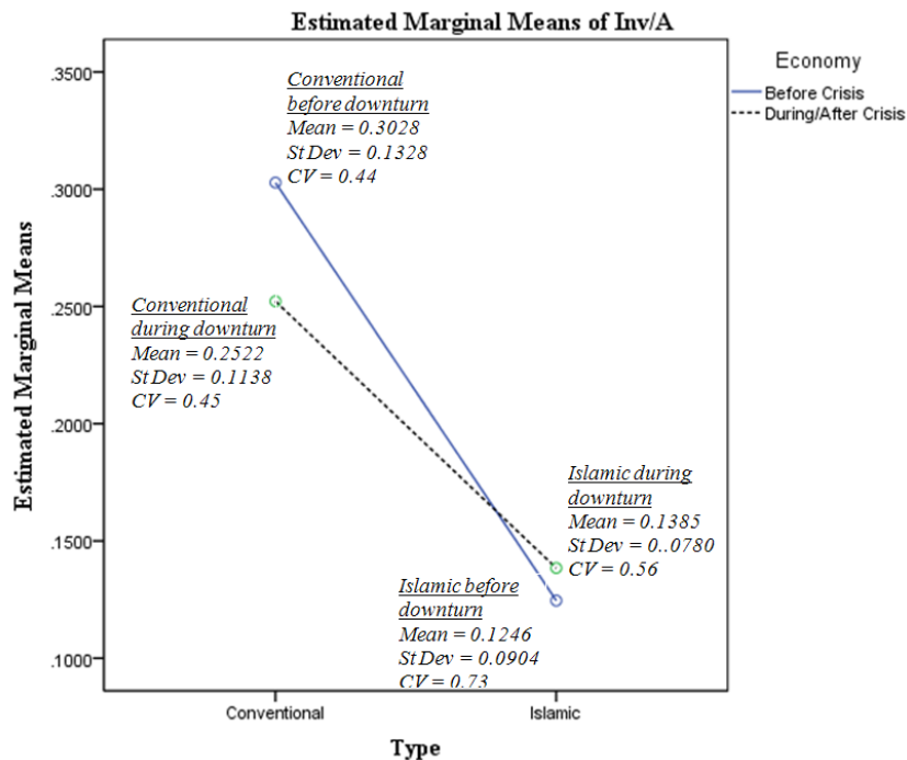
Fig. 1. A profile plot of the interaction effect on Investment/Assets
