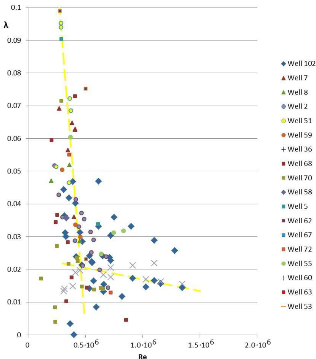
Figure 4 – Distribution of the coefficient of hydraulic resistance between the annular and wellhead pressure
