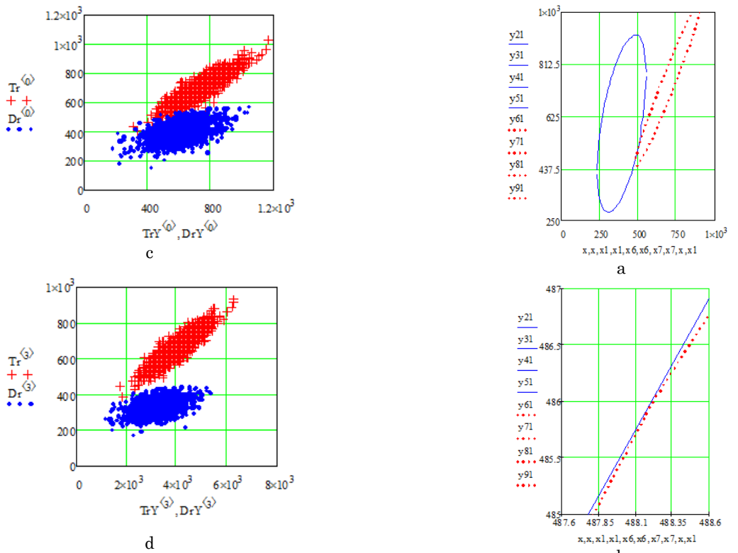
Fig. 1 – Two-dimensional correlation dependences of the Raman polarizing spectrograms of polyester fibers with nanoparticles of silver and without nanoparticles at polarization across and along fibers: a, b – a general view at generation of n = 96 of data for 1 and 4 peaks; c, d – a general view at generation of n = 1536 of data for 1 and 4 peaks
