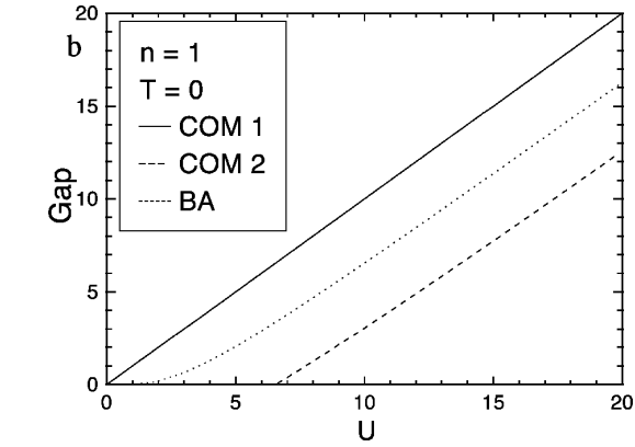
Fig. 1. a) Energy bands for COM 1 (upper panel) and COM 2 (lower panel); b) Energy gap for COM 1, COM 2 and BA (Bethe ansatz).
