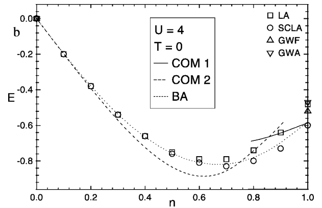
Fig. 2. a) Ground state energy for COM 1 ( E_H ), BA, RG (Renormalization Group), GWF (Gutzwiller wave function), GWA (Gutzwiller approximation), LA (Ladder approximation) and SCLA (Self consistent LA); b) As in (a) for COM 1 ( E_H ) COM 2 ( E_T ), BA, GWF, GWA and LA.
