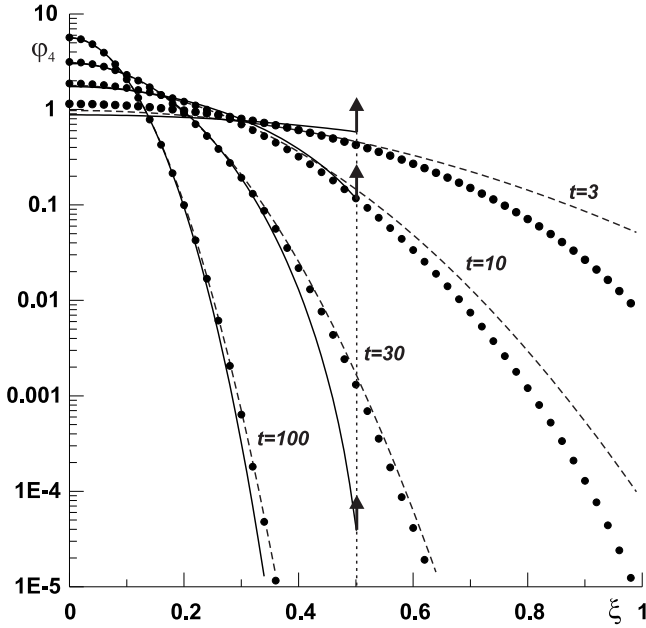
Fig. 3. Same as Fig. 2 for d = 4 .
