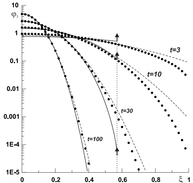
Fig. 2. Distribution density \varphi_d(\xi, t) = p_d(t\xi, t)t for different t . Filled circles present the solution of kinetic equation (7) reconstructed from the moments \mu_0, \mu_2, \dots, \mu_{10} , for d = 3 ; the dashed lines are the solution of the diffusion equation (18) and the solid lines show the solution of the telegraph equation. The vertical arrows indicate the position of the singularity in (16) coinciding with the front positions.
