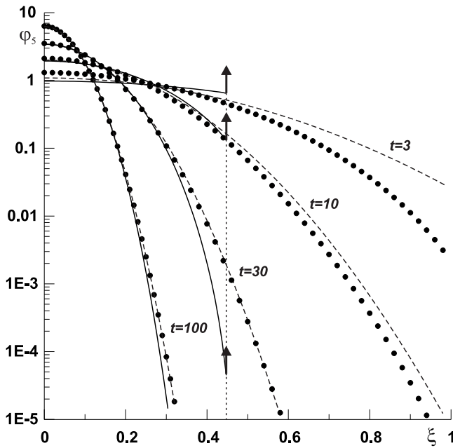
Fig. 4. Same as Fig. 2 for d = 5 .
