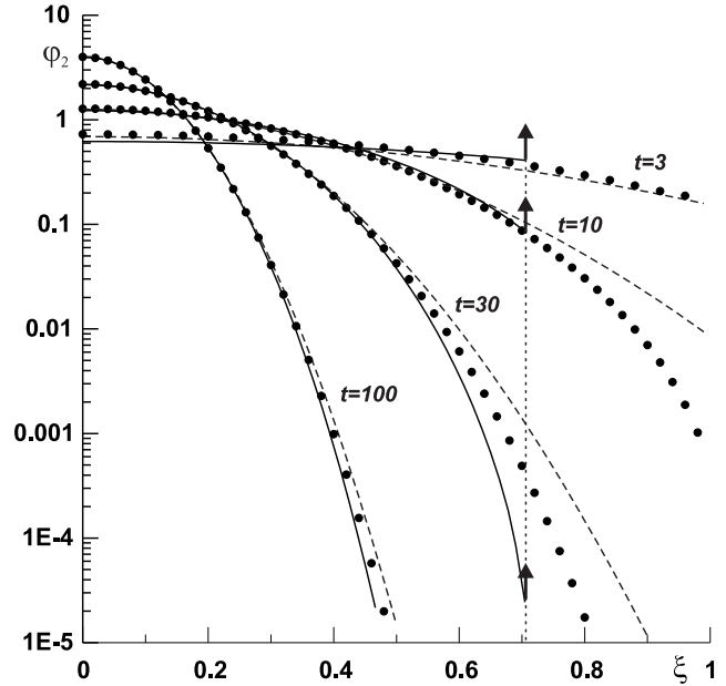
Fig. 1. Distribution density \varphi_d(\xi, t) = p_d(t\xi, t)t for different t . Filled circles present the solution of the kinetic equation (7) obtained by (22) for d = 2 ; the dashed lines are the solution of the diffusion equation (18) and the solid lines show the solution of the telegraph equation. The vertical arrows indicate the position of the singularity in (16) coinciding with the front positions.
