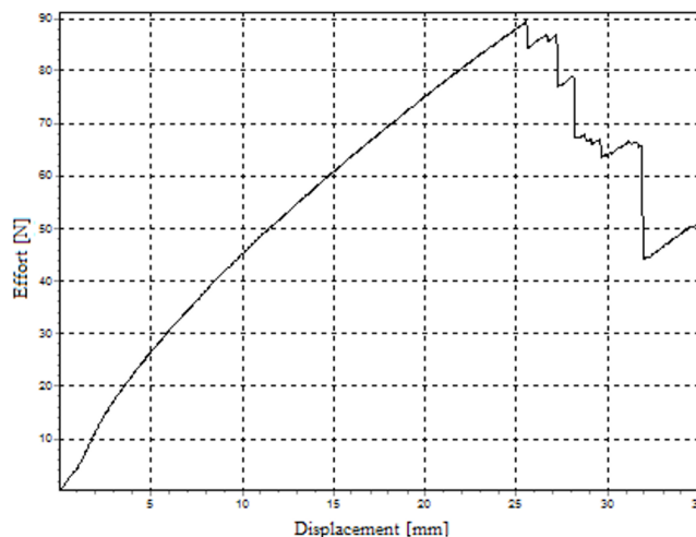
Figure 1. Deformation curve of package paper Fislage
