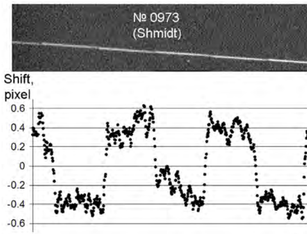
Figure 6: An influence of the Interlace effect on accuracy of the meteor trajectory measurement.
