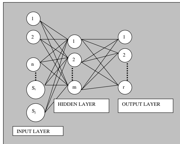
Fig. 2. A Typical Hybrid Neural Network
