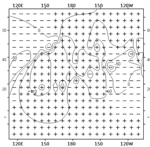
Figure 1. Changing the height of the tropospheric radiowaveguide (see text).
