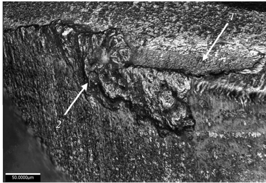
Fig. 3. Condition of cBN 8120 cutting wedge after turning at a feed rate of 0.1 mm/rev: 1 – groove; 2 – peak-up on flank face.
