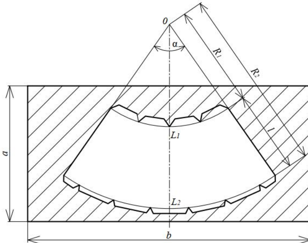
Fig. 1. The scheme of construction of the scan (template) of the change-over from diameter D to diameter d (where a ' b – the size of a standard metal sheet)
