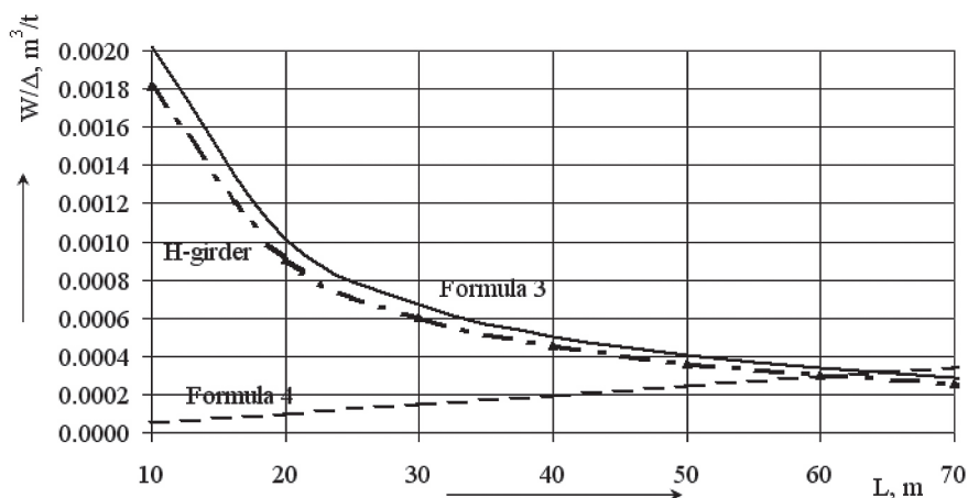
Fig. 5. The value of the relative section modulus.
